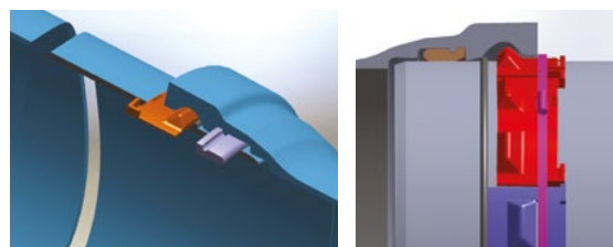
DN 600 - DN 1000
