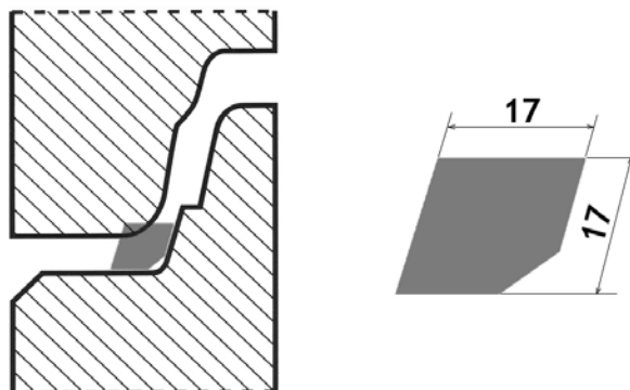
Section diamant
