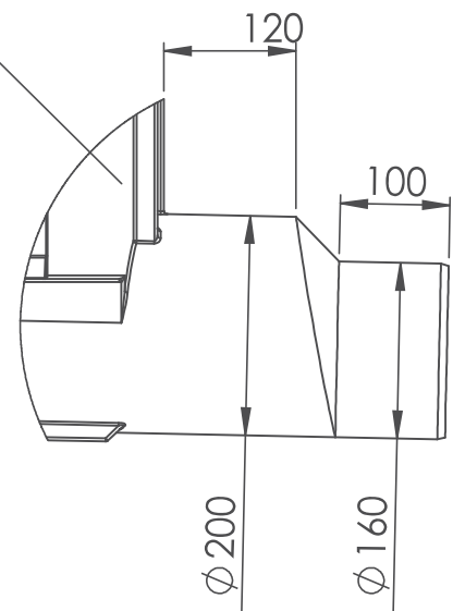
DETAIL A SCALE 1 : 7.5
