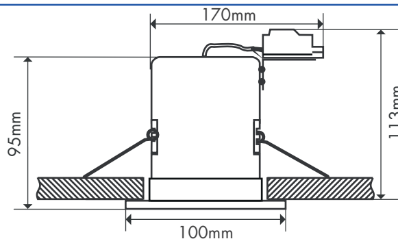
Ref.731604 / 731605 / 731606
