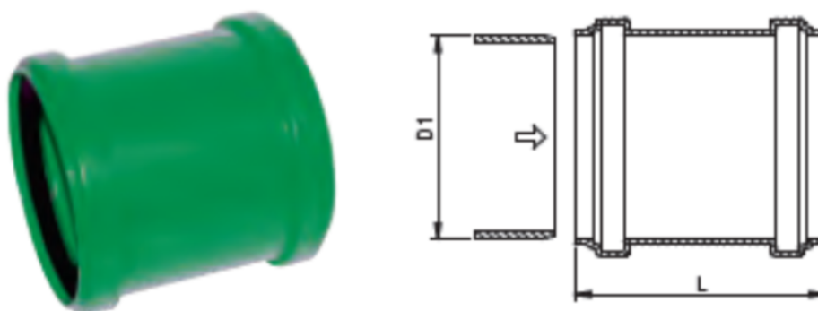
Figure 3.5 : Manchons
