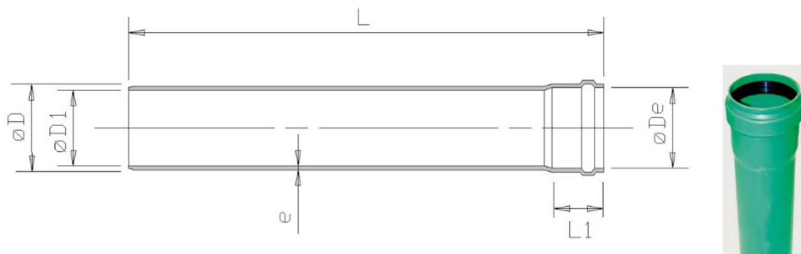
Figure 1 : Tubes KG 2000
