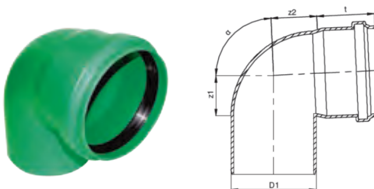
Figure 3.1 : Coudes MF
